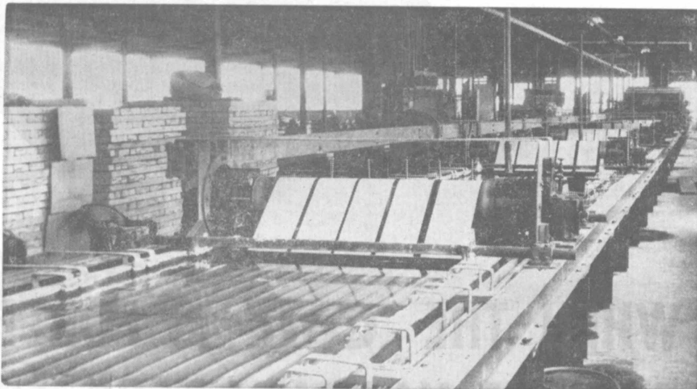
Greer Steel Production Line
